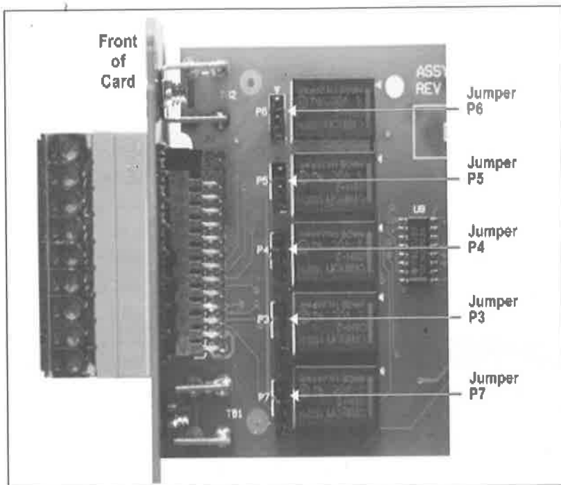
Figure 4.1 Jumper location and numbering
